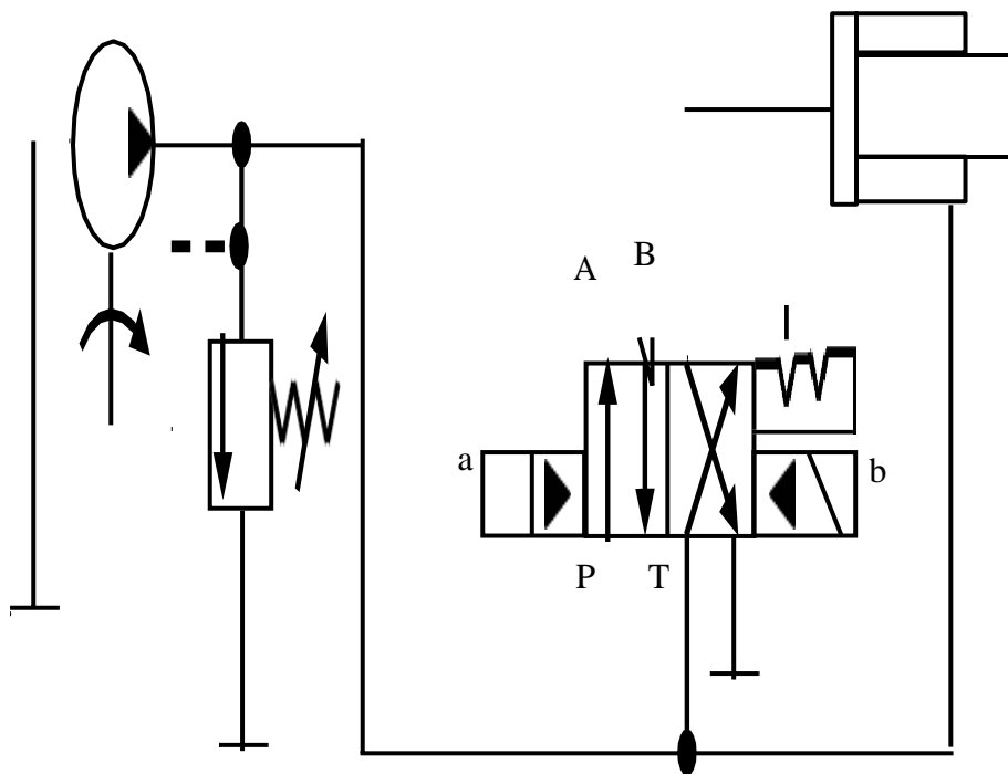
Regenerative Retraction Stroke
