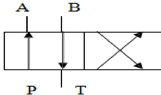
Fig 4 3. 2 / 4 valve symbol
