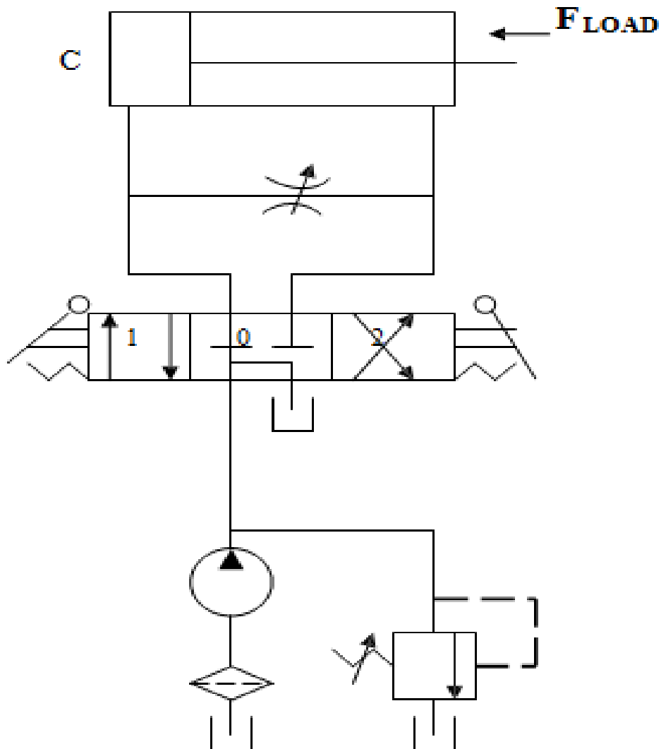
Bleed – Off Circuit.
