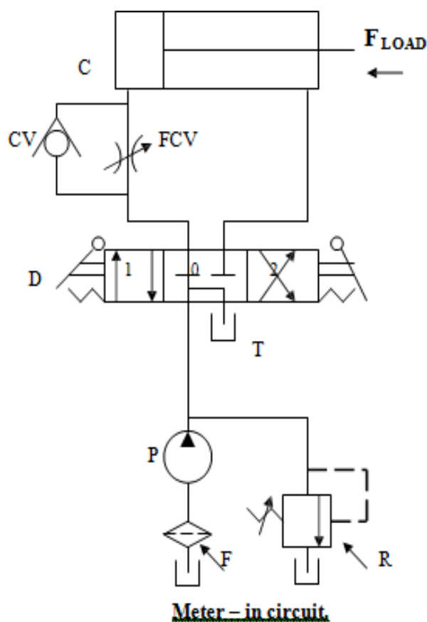
Meter – in Circuit
