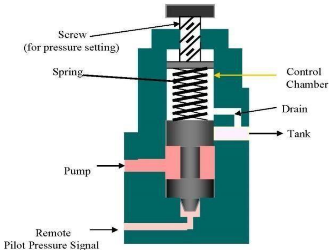
Unloading Valve
