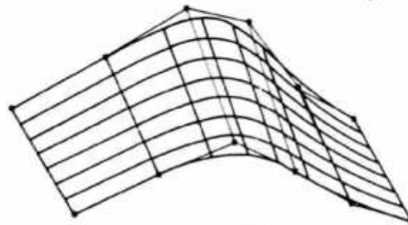
B-spline surface
